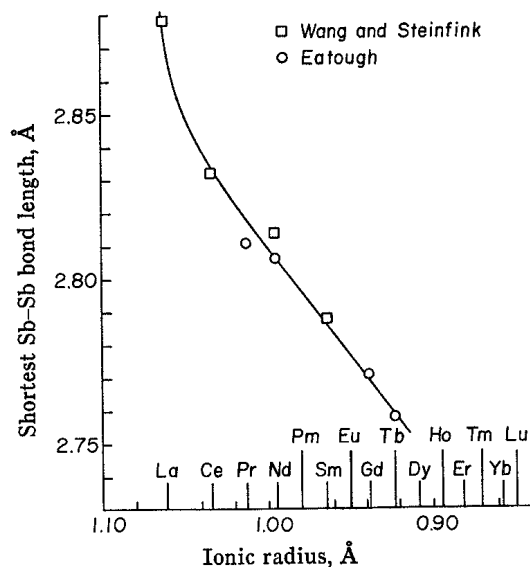
Fig. 2 Short Sb-Sb length in LaSb_2 -type rare earth diantimonides
