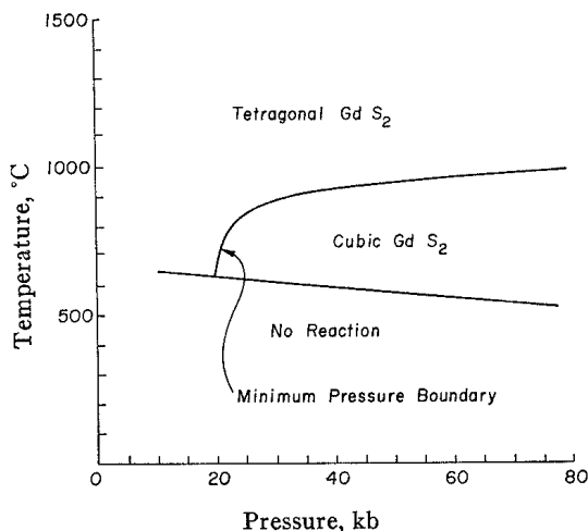
Fig. 3 Reaction product diagram for Gd+2S
