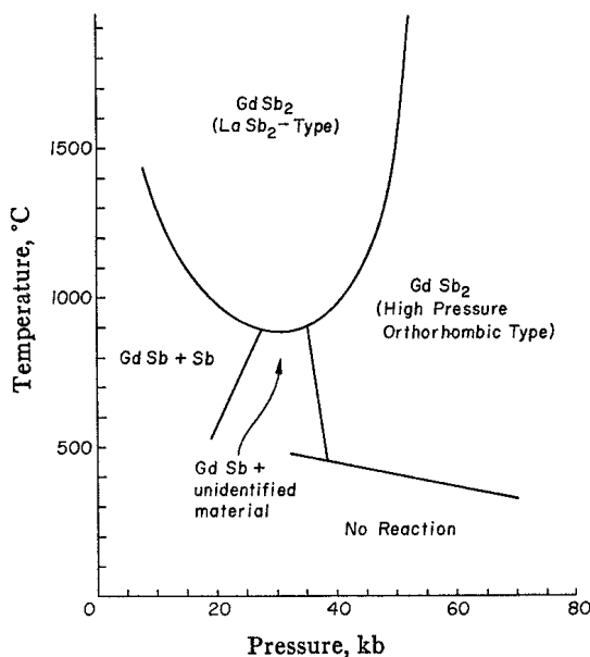
Fig. 1 Reaction product diagram for Gd+2Sb
